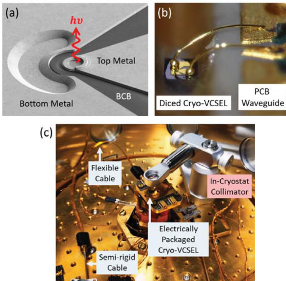
(a) Image of Cryo-VCSEL. (b) VCSEL with wirebond. (c) Low temperature measurement set-up in cryostat. From "Superconducting Processor Modulated VCSELs for 4K High-Speed Optical Data Link." (W. Fu et al. , Article #8000208).
